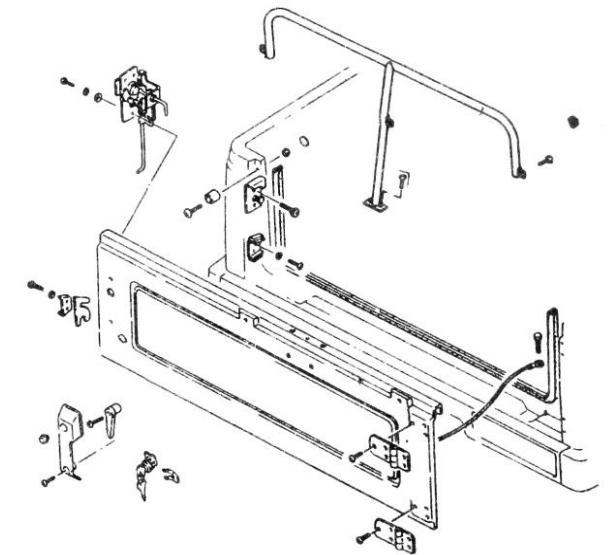
REAR GATE
