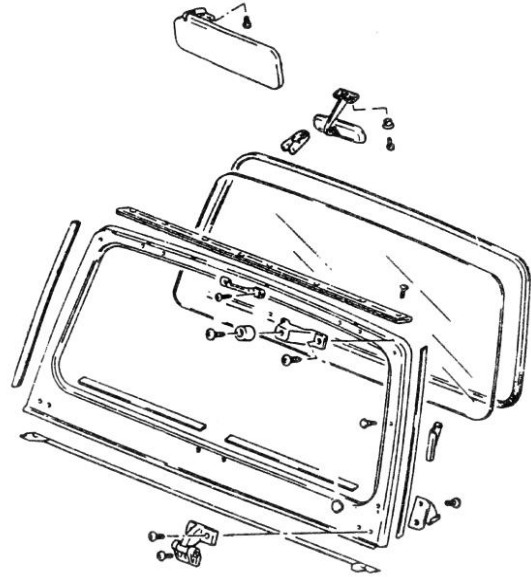
CENTER PANEL
