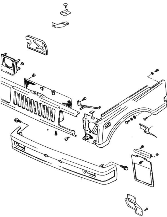
FRONT BODY
