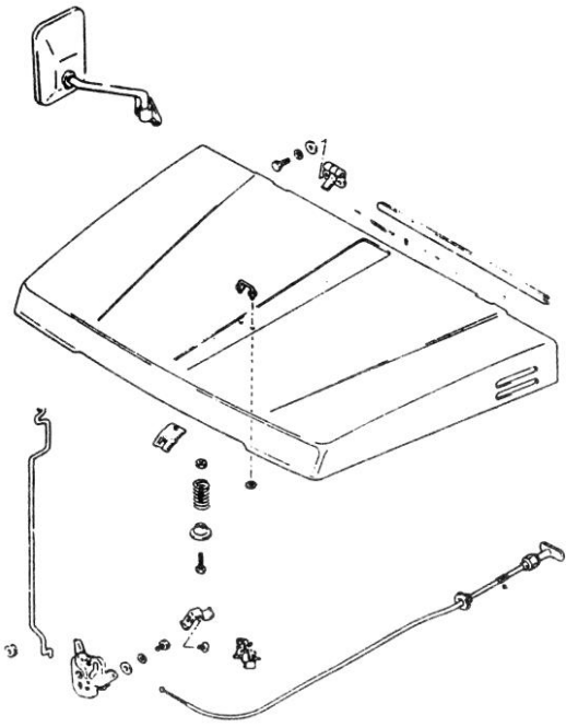
CENTER PANEL
