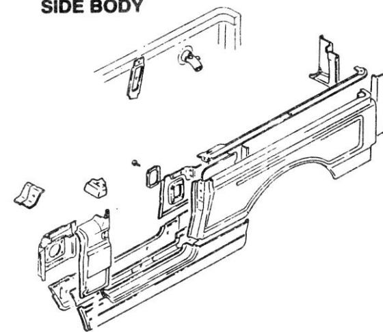
SIDE BODY
